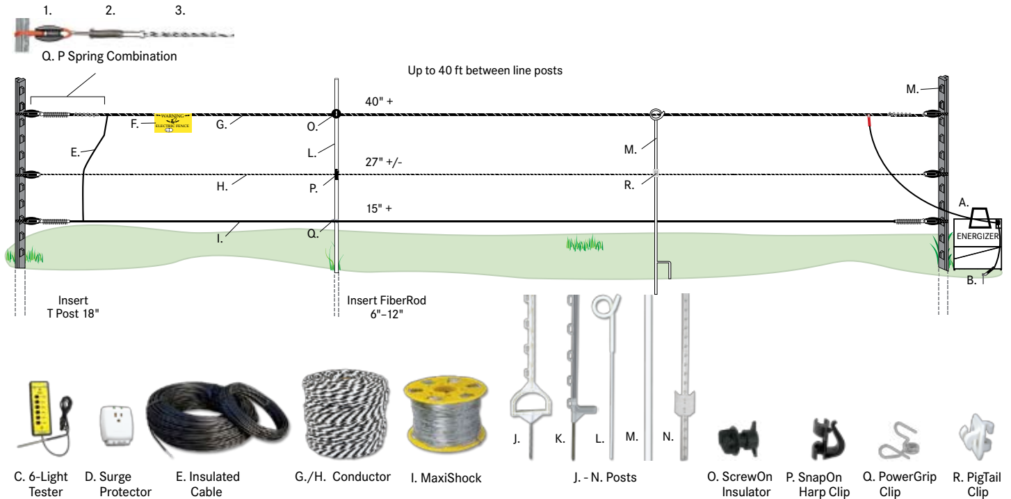
Fence diagram
