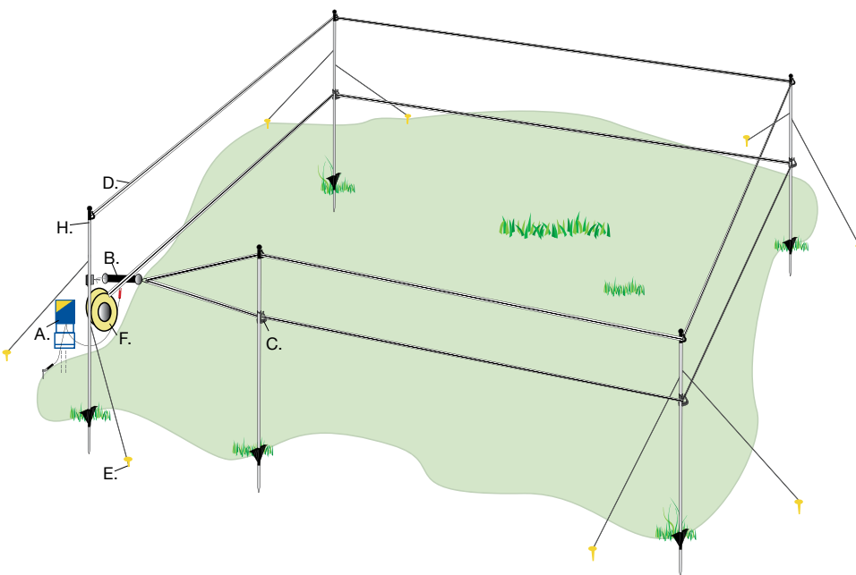
(above) Diagram of a typical (if there is one, because all sites are different) Trailer Paddock Kit layout. The 330 ft of tape provided can create the 2-strand 40 ft x 40 ft (1600 sq ft) paddock shown above, or a 1-strand fence around an 80 ft x 80 ft paddock. (You will need to purchase 4 extra posts if you wish to make the larger paddock.)
