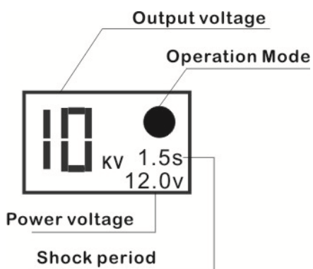
Energizer interface
